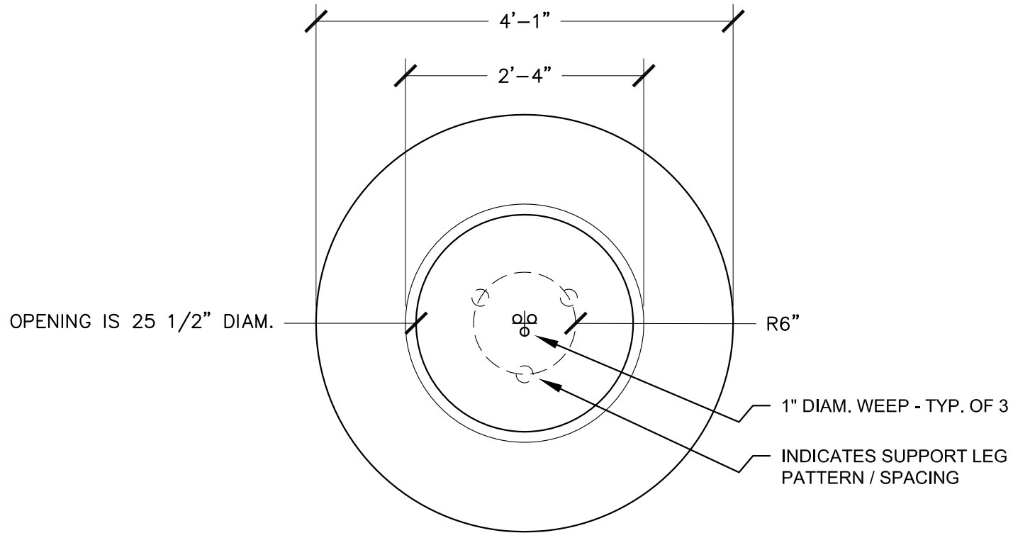
PLAN VIEW
